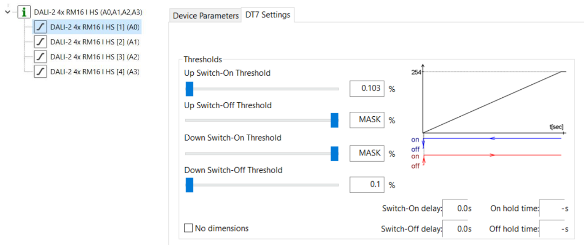
Figure 3 DALI Cockpit, 1. Relay contact, tab: DT7 settings
